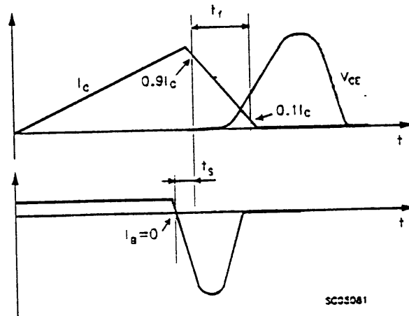
Figure 2: Switching Waveforms in a Deflection Circuit
